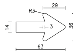
Arrow Detail (NTS)
